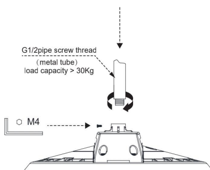
Pipe Mount
